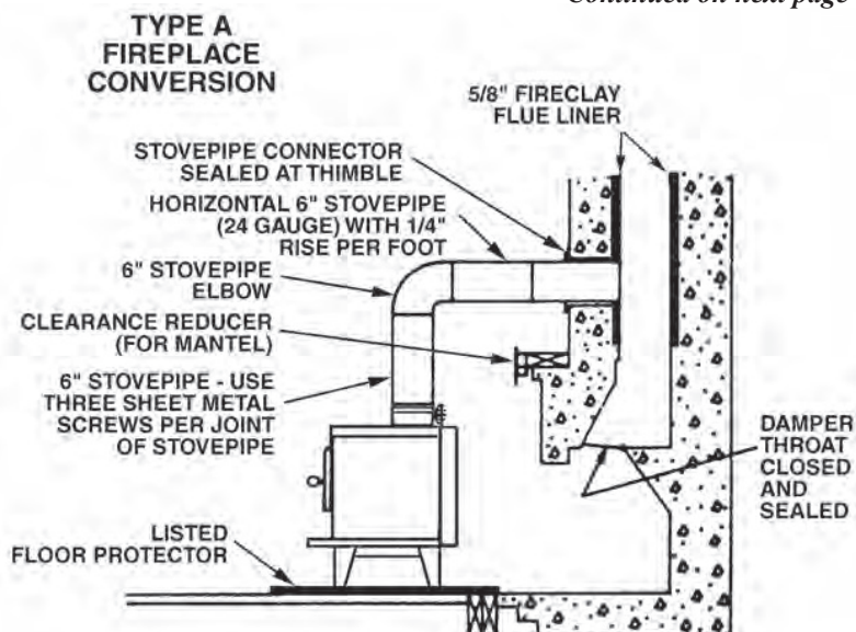
FIG. 15 - Fireplace Conversion
