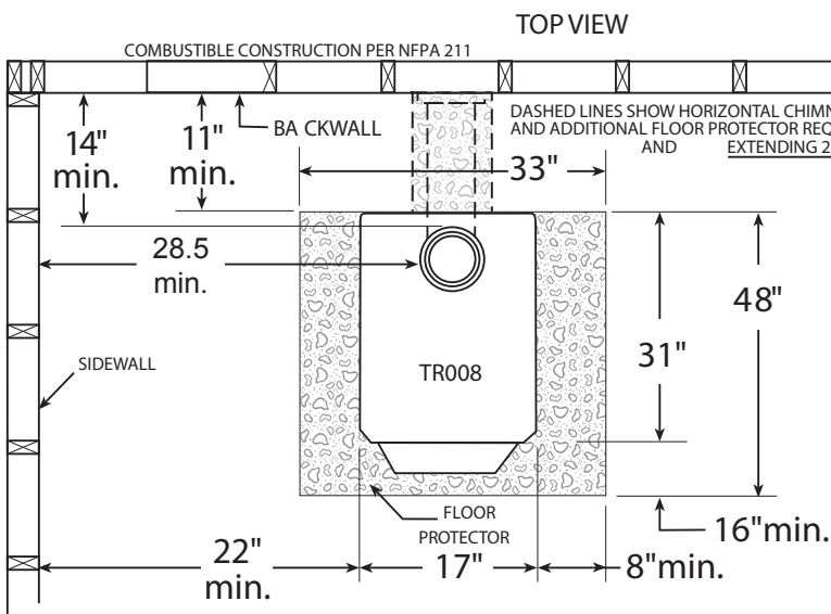
Fig. 5 – Top View Minimum Clearance Dimensions from Combustible Surfaces
