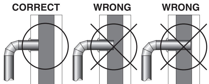
Fig.9 – Stovepipe/Flue Connections
