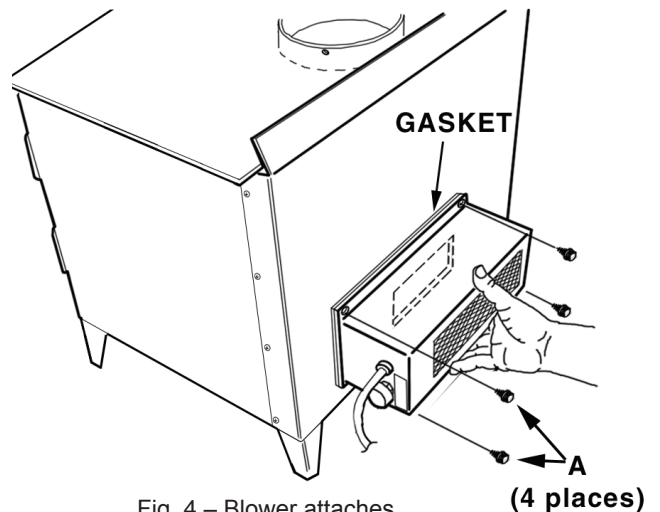
Fig. 4 – Blower attaches to rear heat deflector
