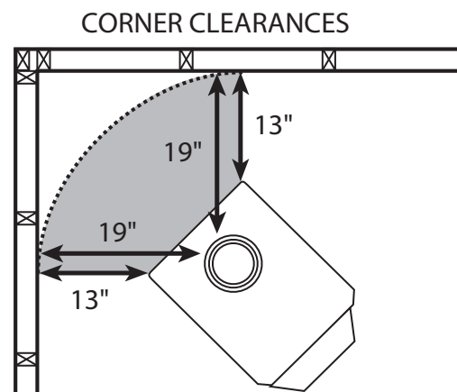
Fig. 6 – Minimum Corner Clearance Dimension from Combustible Surfaces
