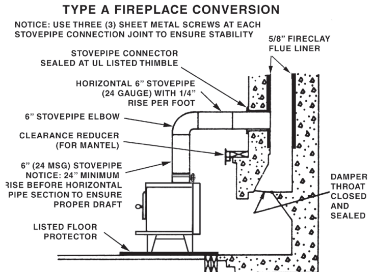
Fig. 14 - Fireplace Conversion
