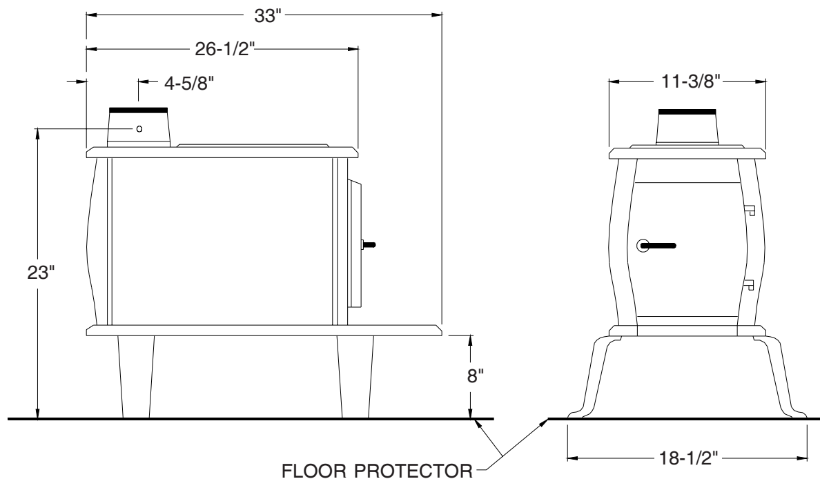
HEATER DIMENSIONS FIG. 1
