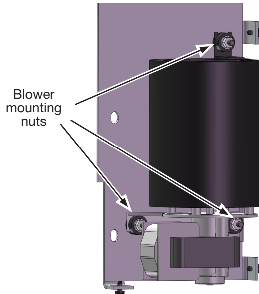
Figure17:TN20.INS.A.fan removal 2.
