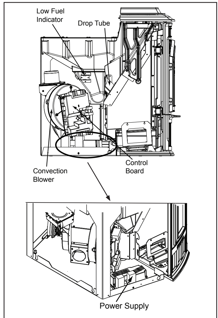
Figure 34.2 - Power Supply, Control Board, Convection Blower
