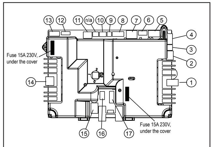
Figure 33.2 - Control Board
