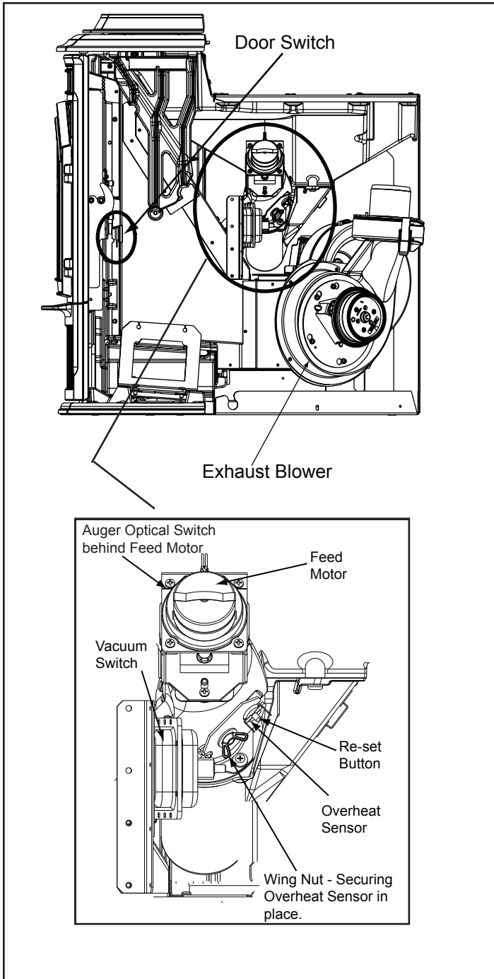
Figure 34.1 - Feed Motor, Vacuum Switch, Exhaust Blower, Overheat Sensor
