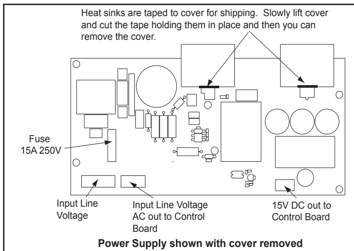
Figure 33.1 - Power Supply
