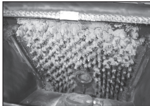
Figure 25.2 - Example of a dirty heat exchanger
