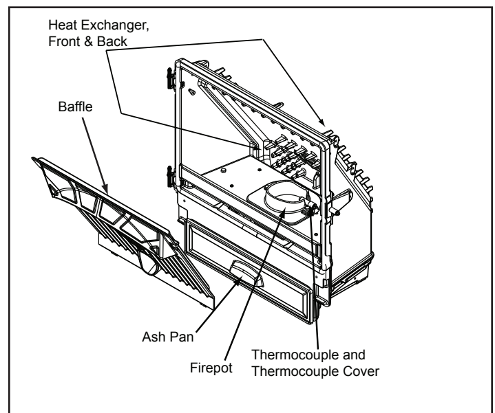
Figure 34.3 - Heat Exchanger, Baffle, Ash Pan, Fire pot Thermocouple & Thermocouple Cover
