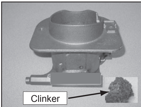
Figure 25.1 - Large Clinker
