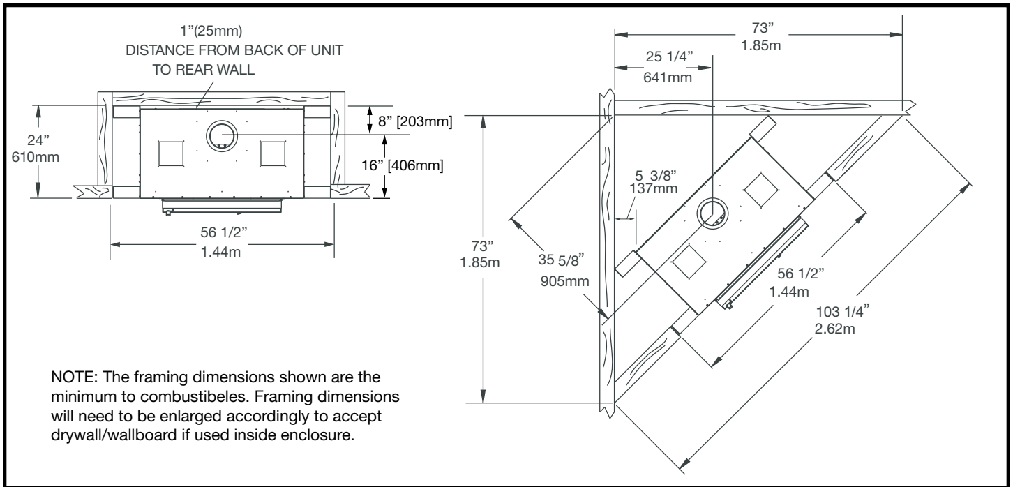
Figure 9: FP30 Framing dimensions. The top front framing must be built as shown, (Figure 10) with no wood framing directly in front of the chimney system
