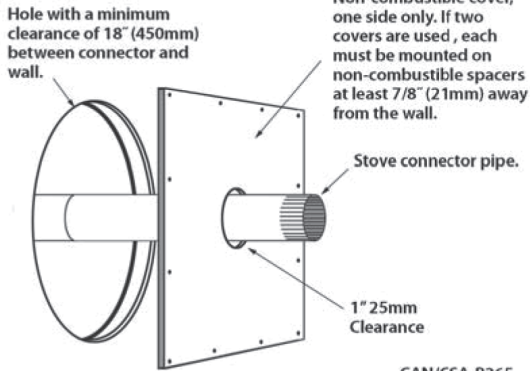
Figure 4 ONLY APPROVED CANADIAN WALL PASS THROUGH
