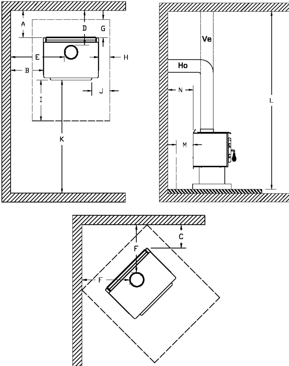
FIGURE 2.3 Clearances to combustibile materials and floor protection
