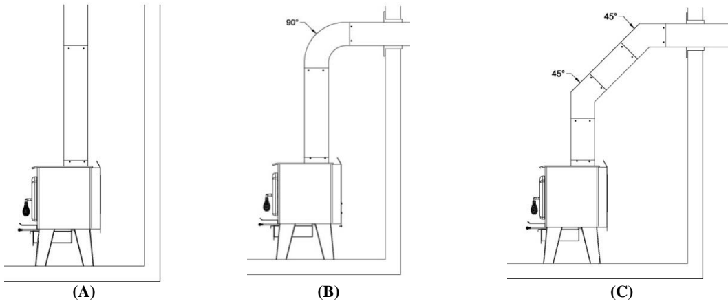
FIGURE 3.4 The use of elbows
