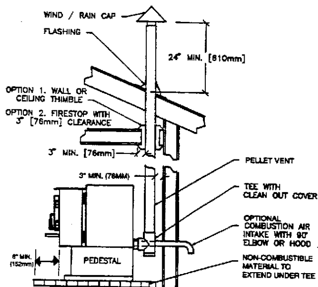
INSIDE VERTICAL INSTALLATION WITH ROOF TERMINATION
