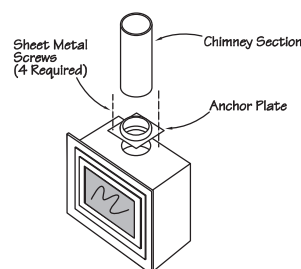
Factory Built Fireplace Installation
