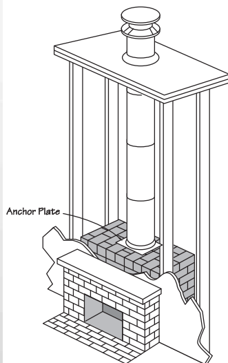
Masonry Fireplace Installation
