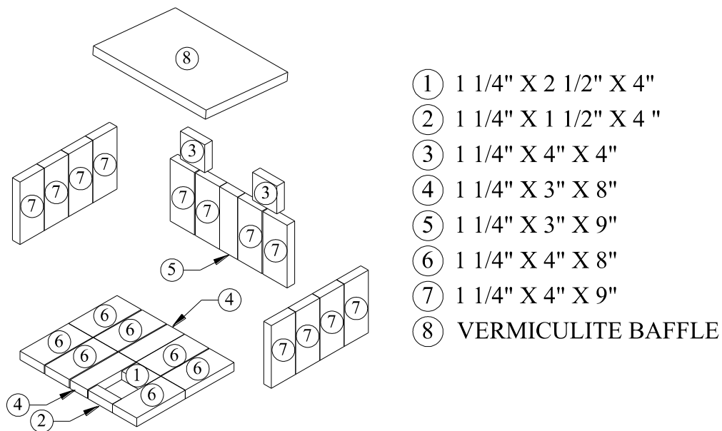
Figure 5.6.2 (B) - Firebrick layout
