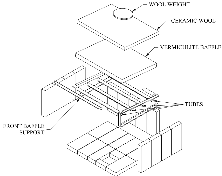
Figure 5.6.2 (A) - Baffle installation
