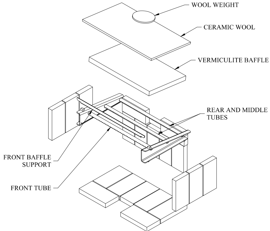
Figure 4.6.1 (A) – Baffle installation for Eastwood 1900
