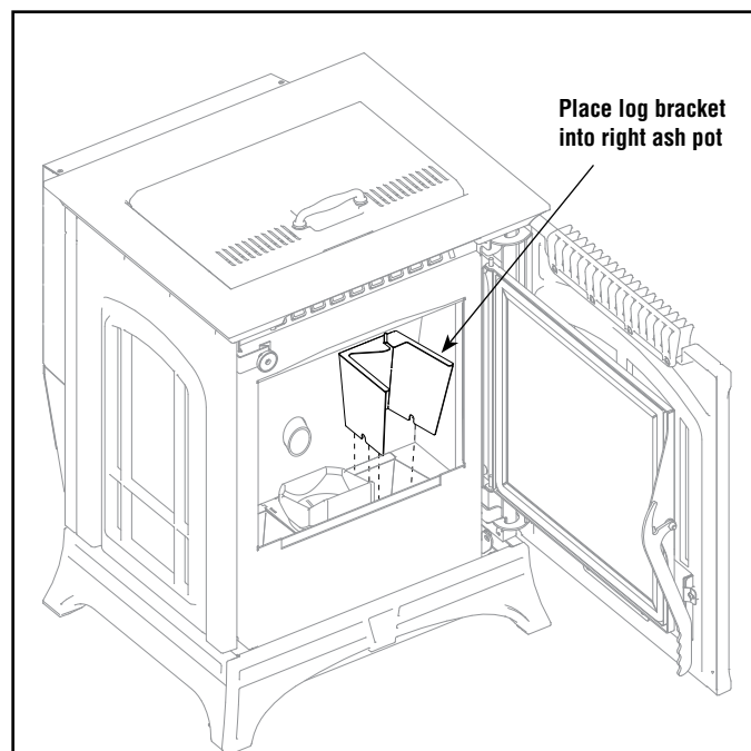
Figure 4 - Install Right Rear Log
