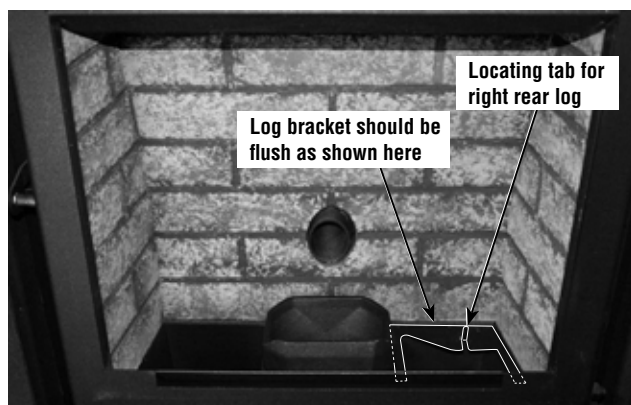
Figure 3 - Install Log Bracket
