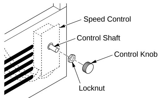
Figure 11 - Attaching Speed Control to Firebox
