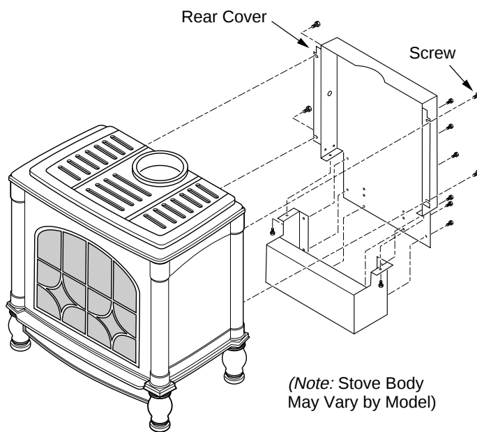
Figure 22 - Removing/ Installing Rear Cover
