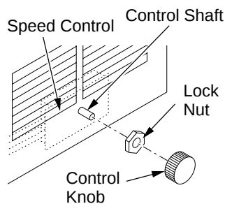
Figure 3 - Attaching Speed Control
