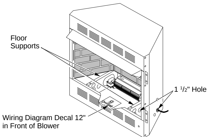
Figure 12 - Location of Wiring Diagram Decal
