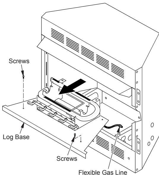
Figure 1 - Removing Log Base from Fireplace
