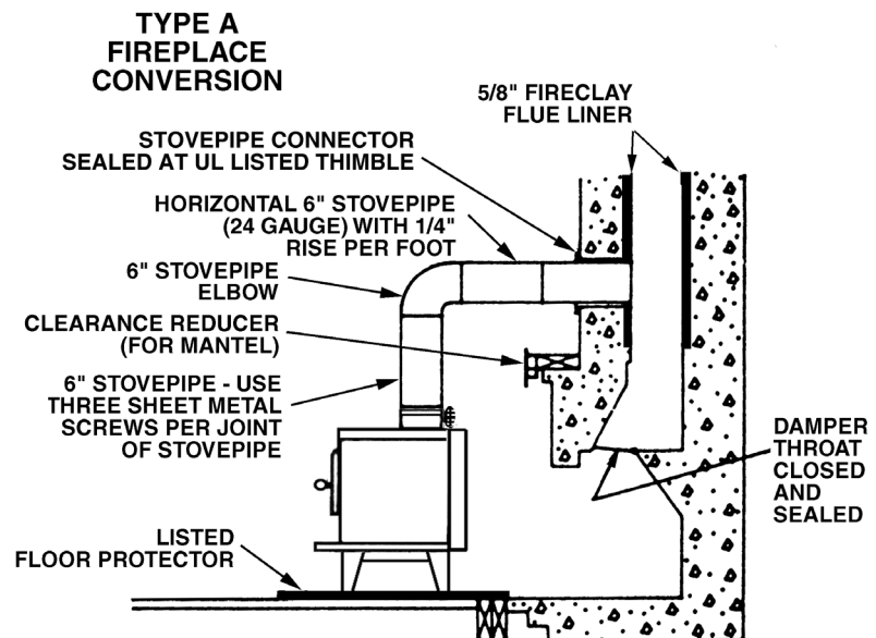
Fig. 12 - Fireplace Conversion
