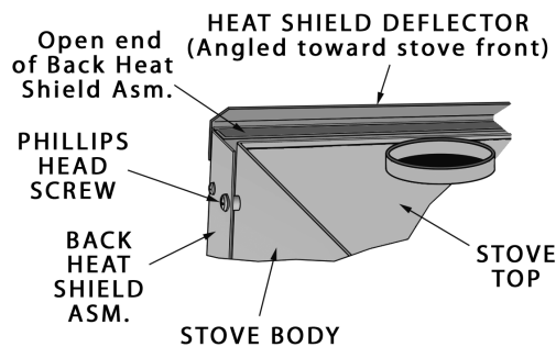
Fig. 2 – TOP VIEW
